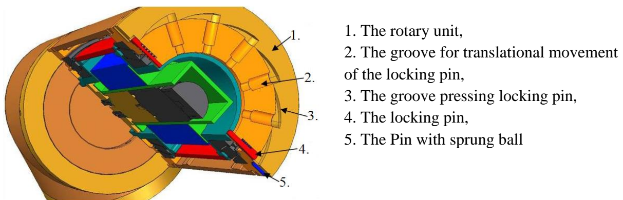
Figure 2. Components of the locking system
