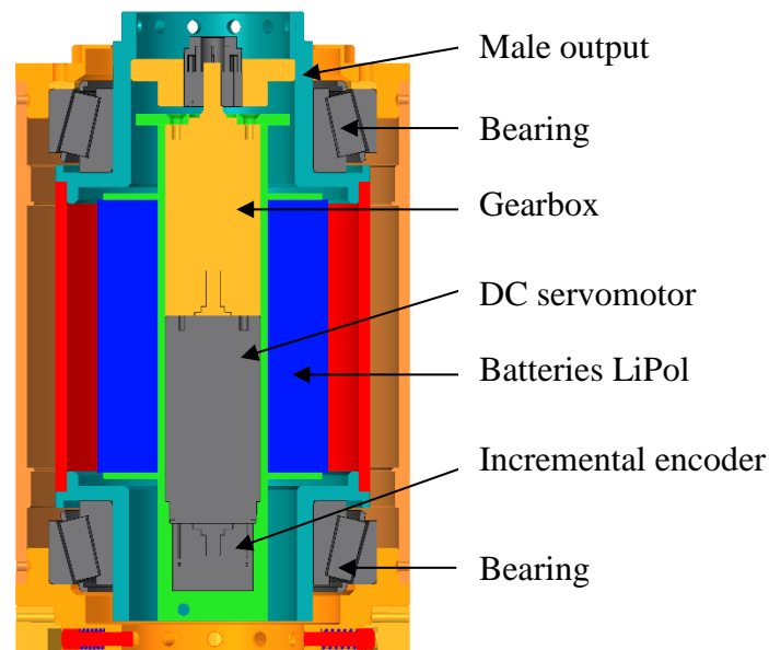
Figure 1. Cut the Rotation Universal Module flesh
