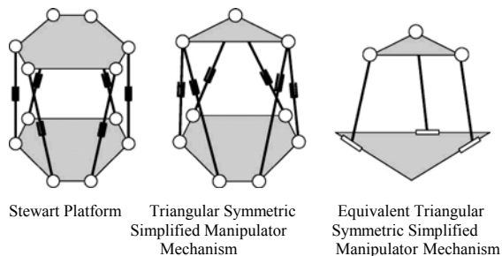
Figure 2 General parallel manipulators
