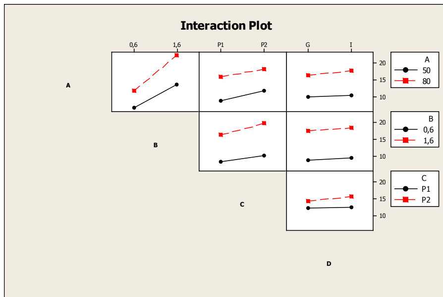
Figure 4 Interaction plot
