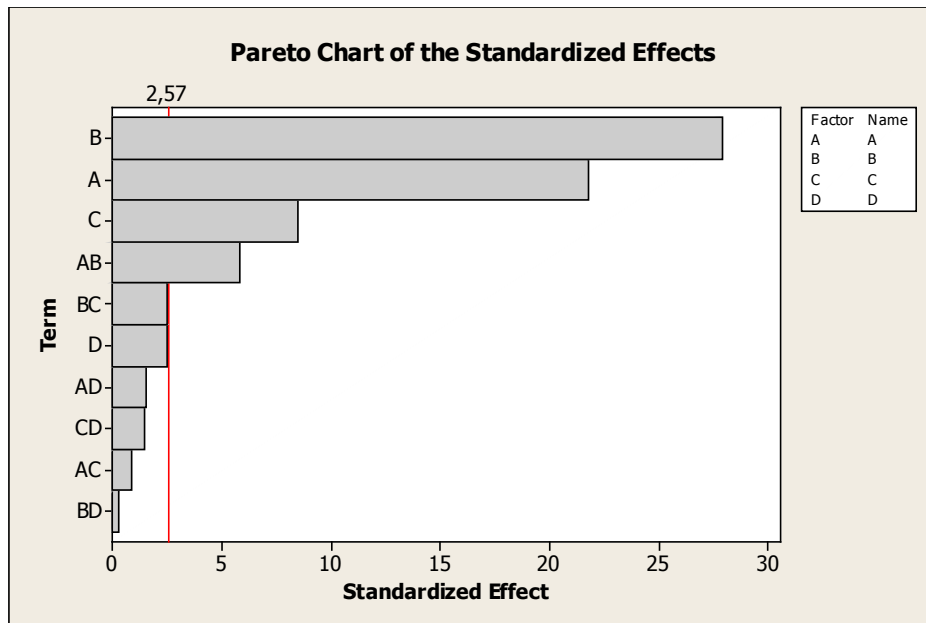
Figure 2 Pareto chart
