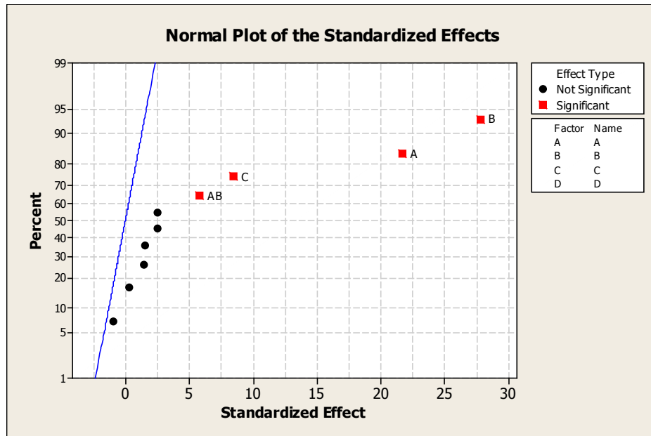
Figure 3 Normal probability plot
